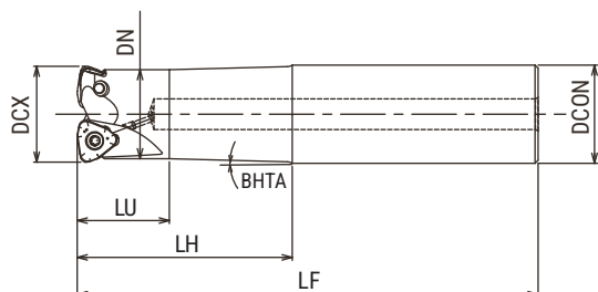
Fig.1 DCX=Ø32
