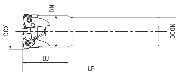
Fig.2 DCX=Ø35, 40
