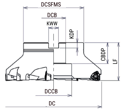
Fig.2 Without coolant hole
