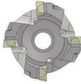
4 inserts SKG-4050R-10-22
