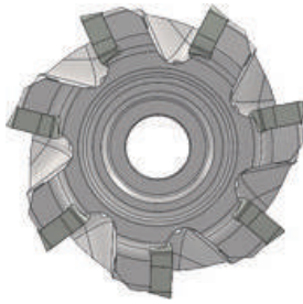
7 inserts SKG-7050R-09-22
