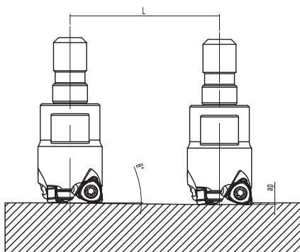
Ramping
