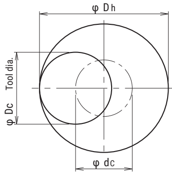
Helical interpolation
