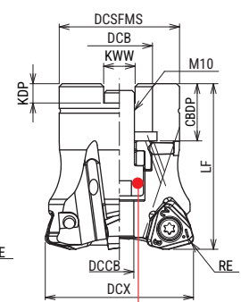
Fig.3 Through coolant hole
