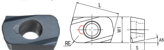
For high hardened steel (EPHW1003 * * ZTR)
