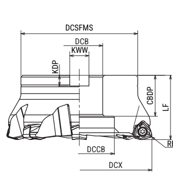
Fig.2 Without coolant hole
