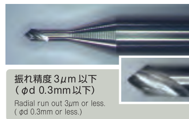
60SPA刃先形状 Cutting edge of 60SPA
