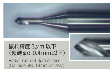
60SPC-CB刃先形状
