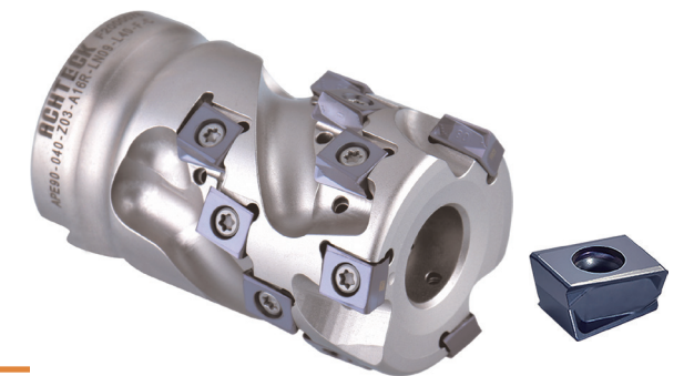
Application: Profile/main hole rough milling Solution: Achteck porcupine milling cutter APE90-LN09/13/AO12
