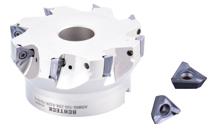
Application: Pocket rough milling Solution: Achteck TDMT 1505 series
