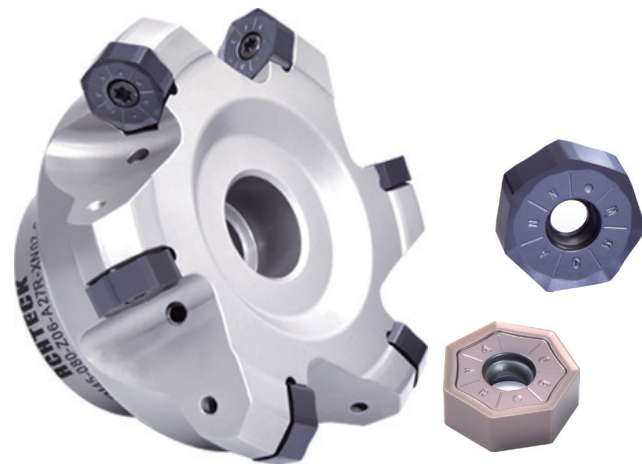
Application: Rough face milling Solution: Achteck XNMU 07 /09 series
